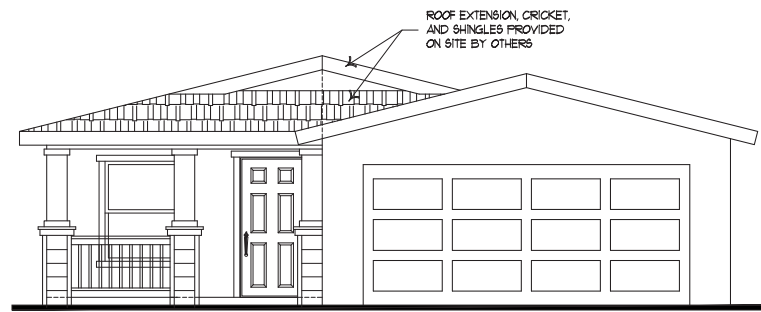
PORCH ENDWALL (SHOWN W/ SITE-BUILT GARAGE)
