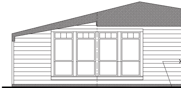
PORCH ELEVATION
