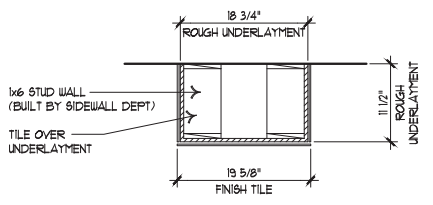
SIDEWALL PLANT-ON COLUMN
