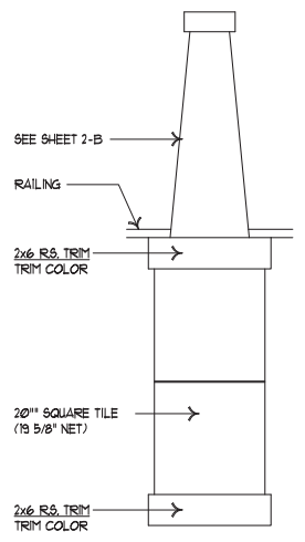
COLUMN ELEVATION
