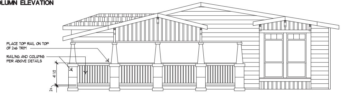
COLUMN ELEVATION
