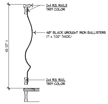
PORCH RAIL
