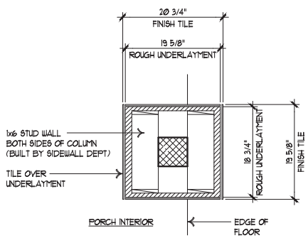
PORCH COLUMN
